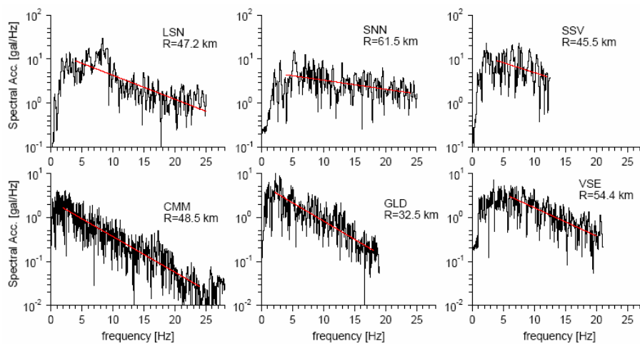
Figure 9. Estimates of k from acceleration NS components recorded during the October 31 main shock at stations CMM, GLD, VSE, LSN, SNN and SSV. Frequency bandwidths for regressions were chosen according to the corner frequency of the event and the high frequency noise of data.
