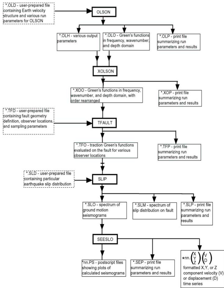
Figure 1.3 - Operative scheme of COMPSYN
