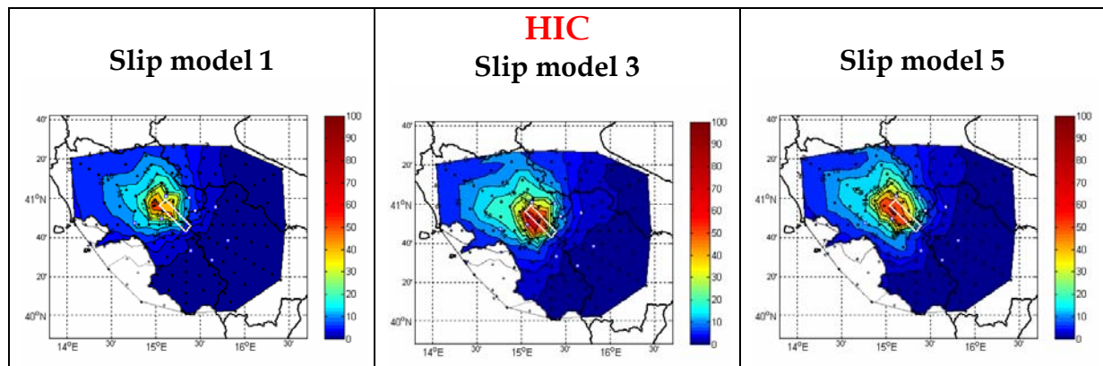
Figure 4.5 - PGV maps computed with DSM (top) and Hic (bottom) techniques considering different K 2 slip model.
