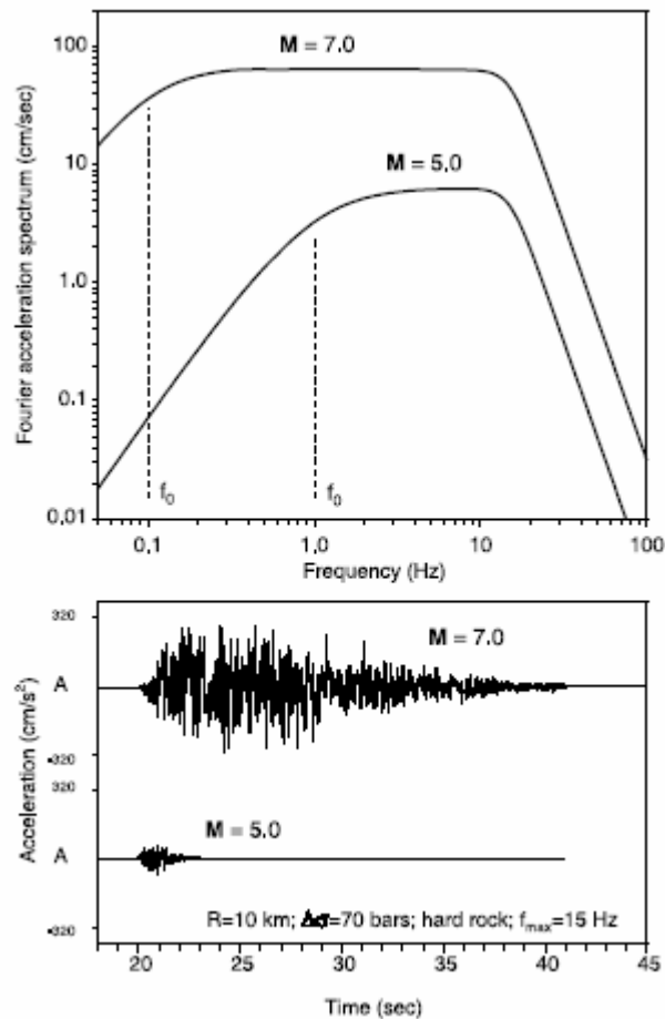
Figure 1.1 - Basis for stochastic method (from Boore 2003). Radiated energy described by the spectra in the upper part of the figure is assumed to be distributed randomly over a duration equal to the inverse of the lower corner frequency ( f_0 ). Each time series is one realization of the random process for the actual spectrum shown. When plotted on a log scale, the levels of the low-frequency part of the spectra are directly proportional to the logarithm of the seismic moment and thus to the moment magnitude. Various peak ground-motion parameters (such as response spectra, instrument response, and velocity and acceleration) can be obtained by averaging the parameters computed from each member of a suite of acceleration time series or more simply by using random vibration theory, working directly with the spectra.
