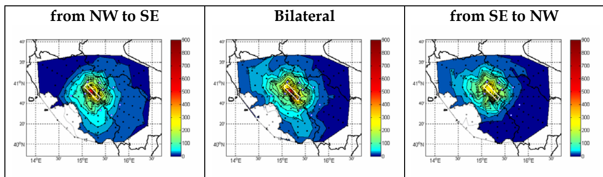
Figure 4.4 - PGA maps computed with HIC technique considering different position of the nucleation point (rupture velocity = 2.9 km/s).
