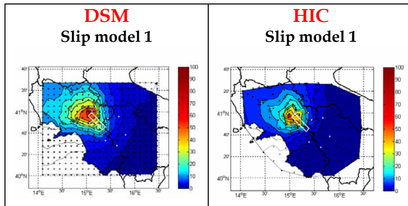
Figure 4.1 - PGV maps computed with DSM (left) and HIC (right) techniques for the same rupture model (slip model 1, rupture velocity=2.7 km/s).
