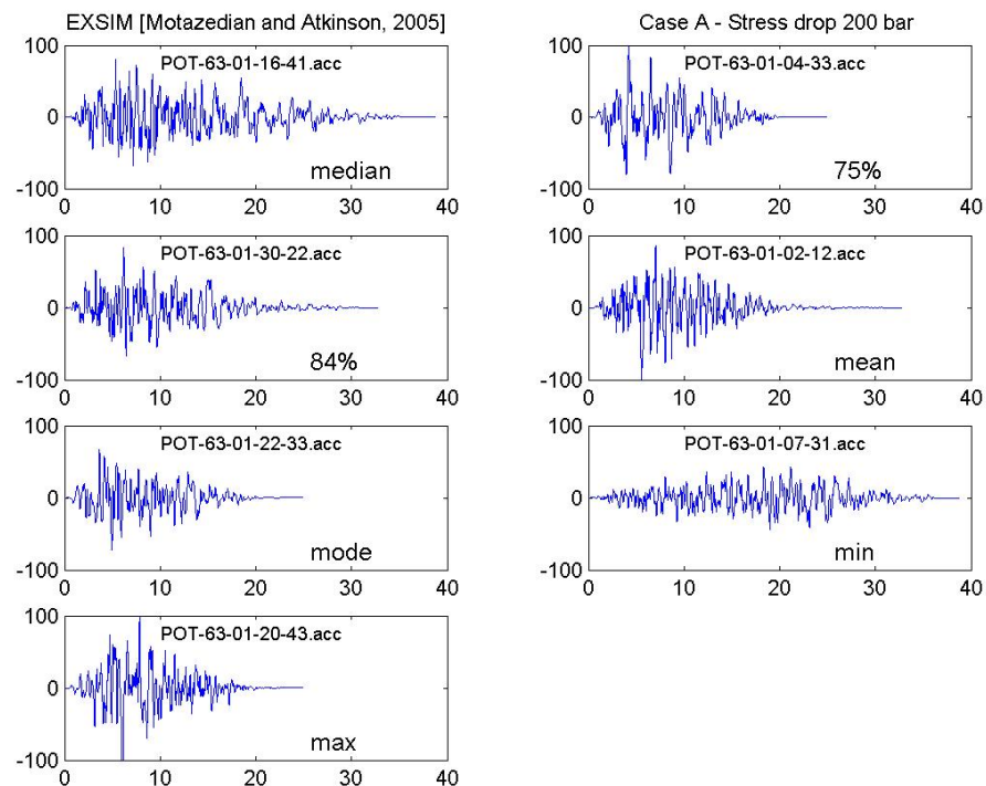
Figure 4. Fault F8 (Andreatta Filano): plots of the simulated time series associated to the statistical values of PGA corresponding to the median, 75% percentile, 84 % percentile, mean, mode, minimum and maximum.
