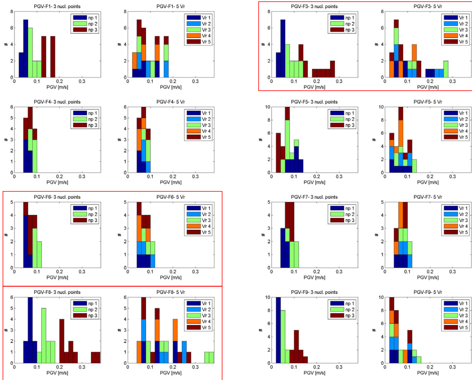
Figure 3.5. PGV variability (nucleation points – Rupture velocity). Red boxes indicate the faults which produce the maximum shaking scenario at Potenza.
