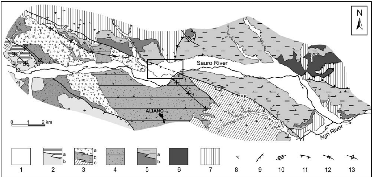
Figure 2.3.1. Scorciabuoi fault
