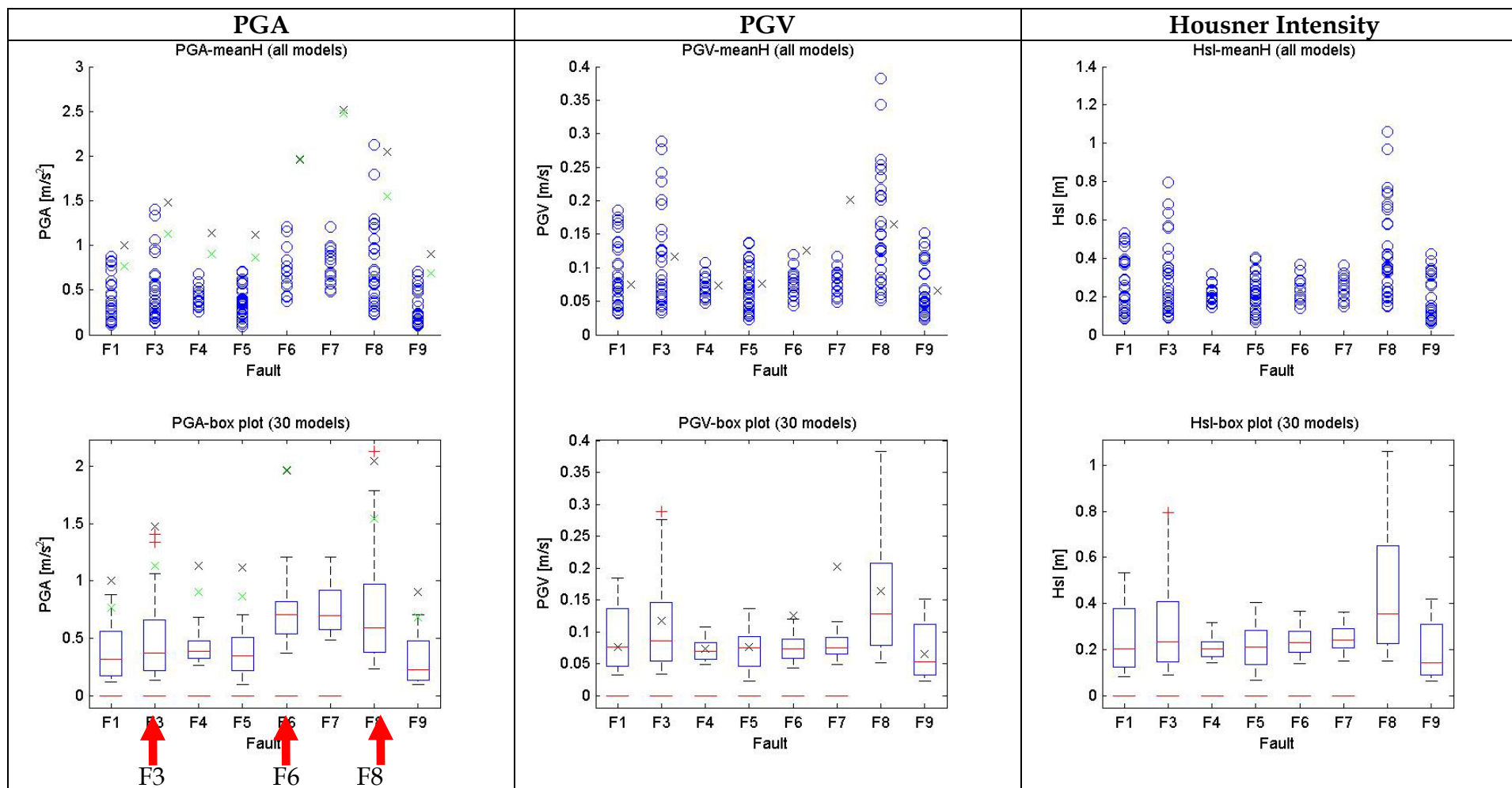
Figure 3.4. PGA, PGV, and Housner Intensity for the simulated faults. The tops and bottoms of each "box" are the 25 th and 75 th percentiles of the samples (i.e. interquartile ranges). The line in the middle of each box is the sample median. The "whiskers" are lines extending above and below each box to show the extent of the rest of the data. Observations beyond the whisker length are marked as outlier (by default, an outlier is a value that is more than 1.5 times the interquartile range away from the top or bottom of the box). Outliers are displayed with a red + sign). Crosses are the values from empirical models at magnitude and fault distance corresponding to each fault (black -Sabetta and Pugliese, 1996; green - Ambraseys et al., 2005).
