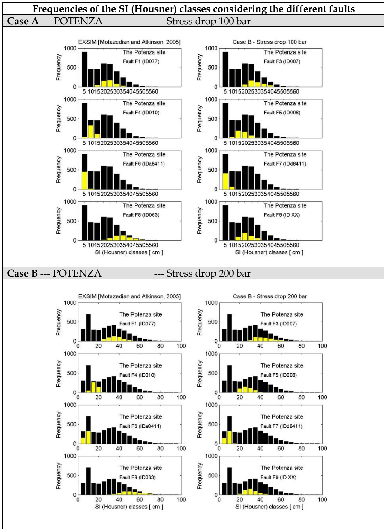
Figure 3.4.2 Comparisons of the frequency versus SI (Housner) class graphs considering the 3,840 time series produced from all of the faults (black bars) and considering the 480 time series from each single fault (yellow bars). The results from the different values of stress drop (100 and 200 bar) are shown.
