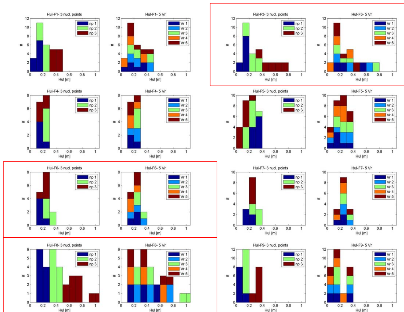
Figure 3.6. Housner Intensity computed between 0.1 and 2.5 seconds: variability due to nucleation point position and rupture velocity. Red boxes indicate the faults which produce the maximum shaking scenario at Potenza.
